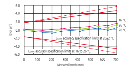
Graph showing the effectiveness of temperature compensation
