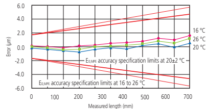
Graph showing the effectiveness of temperature compensation
