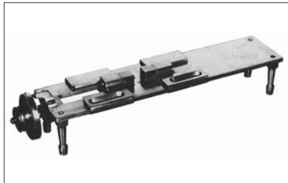
Maudslay's "Lord Chancellor" a table-top micrometer
