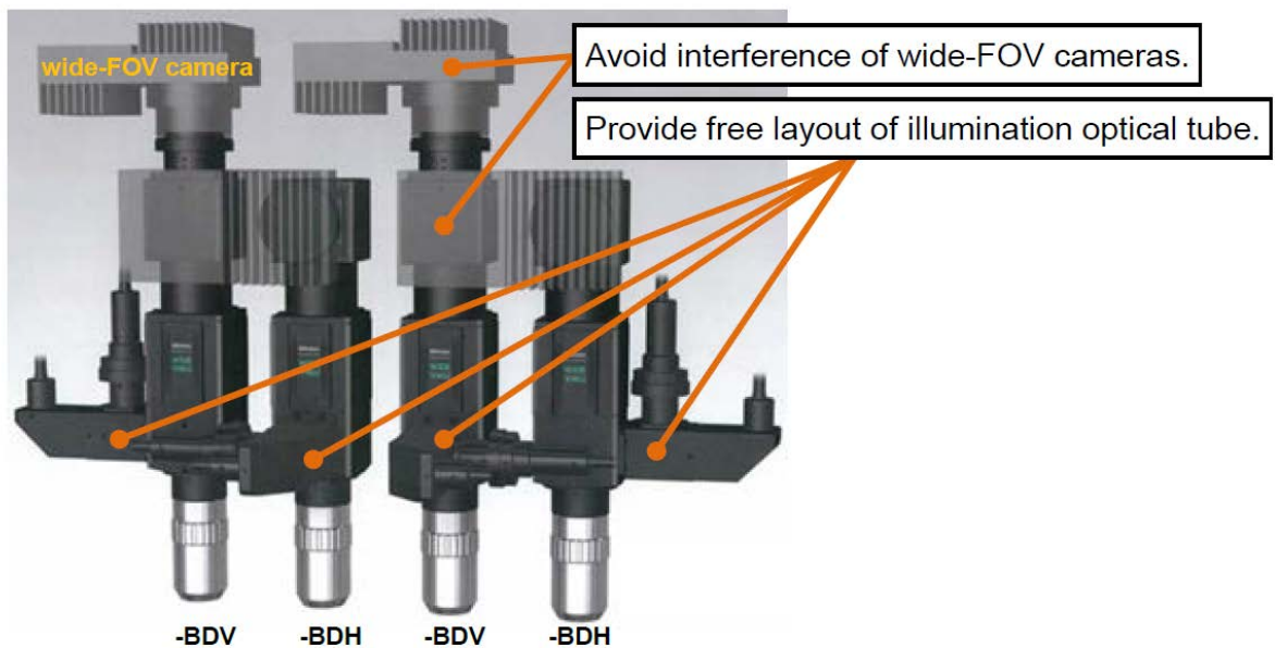
Fig. 1 Illustration of Combining Multiple Wide-FOV VMU
